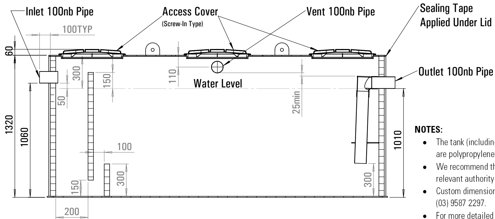
SECTION B-B
