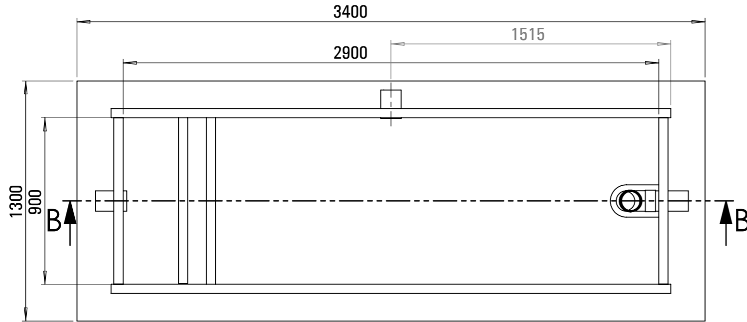
Top View without Lid
