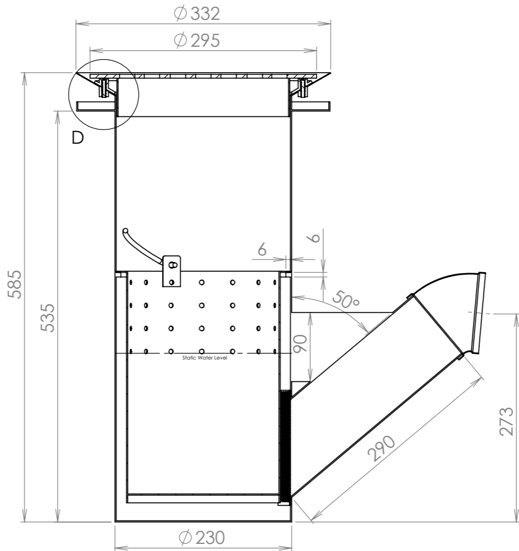
SECTION C-C
