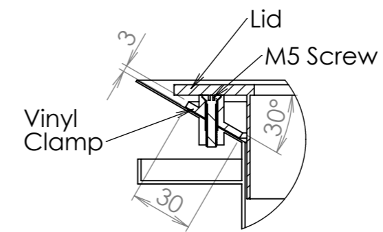
DETAIL D SCALE 2 : 5
